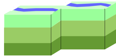
Figure 5-1: Types and Characteristics of Earthquake Faults in Southern California
